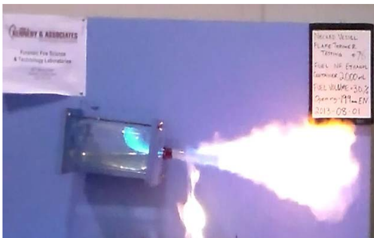
Figure 1. Necked Vessel Flame Thrower Effect test at JAK&A Laboratories.
